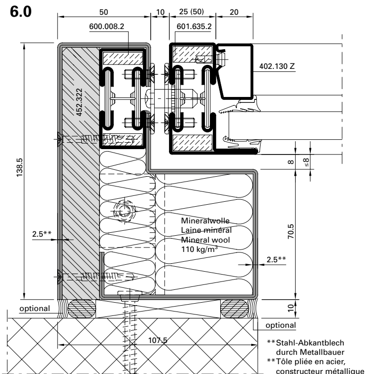
DXF DWG 31-0501-C-010
